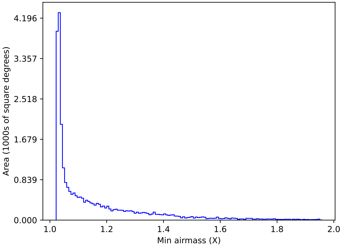
weather_cloudso31v3.4_10yrs Yr 1 all bands: Min airmass
