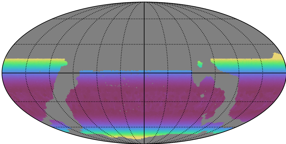
weather_cloudso31v3.4_10yrs WFD z band: Min airmass
