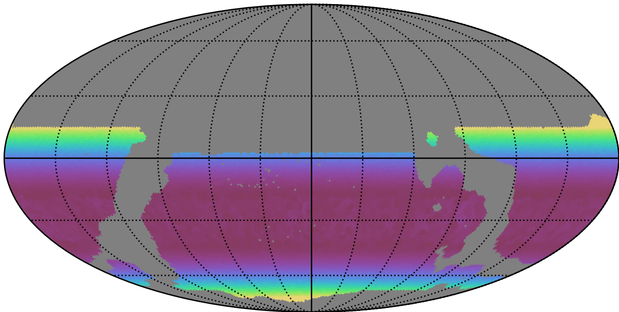
weather_cloudso31v3.4_10yrs WFD y band: Min airmass
