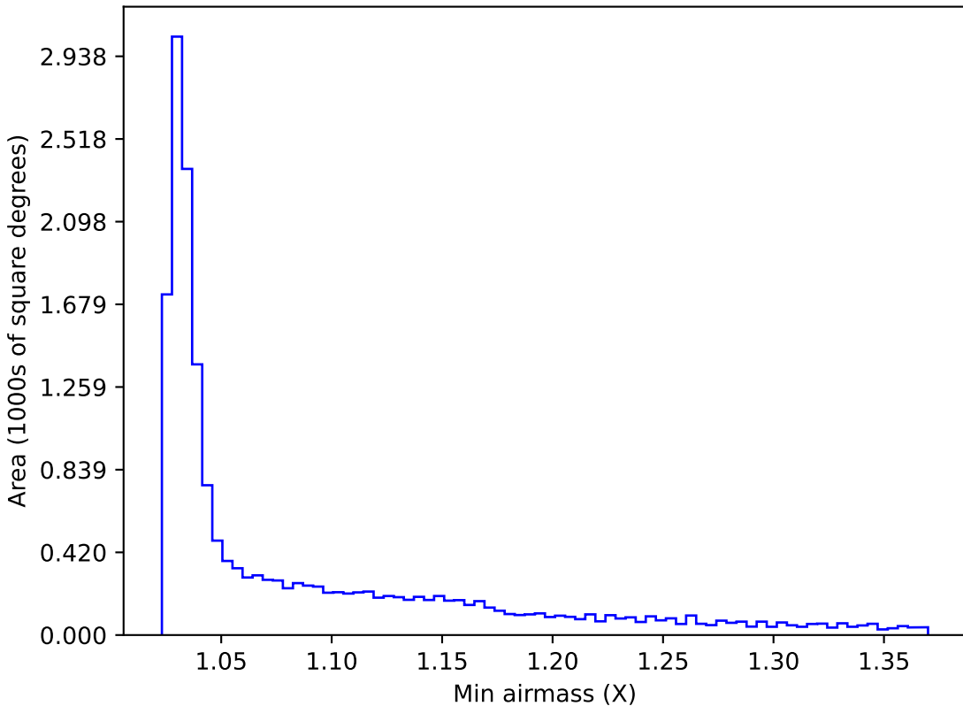
weather_cloudso31v3.4_10yrs WFD y band: Min airmass
