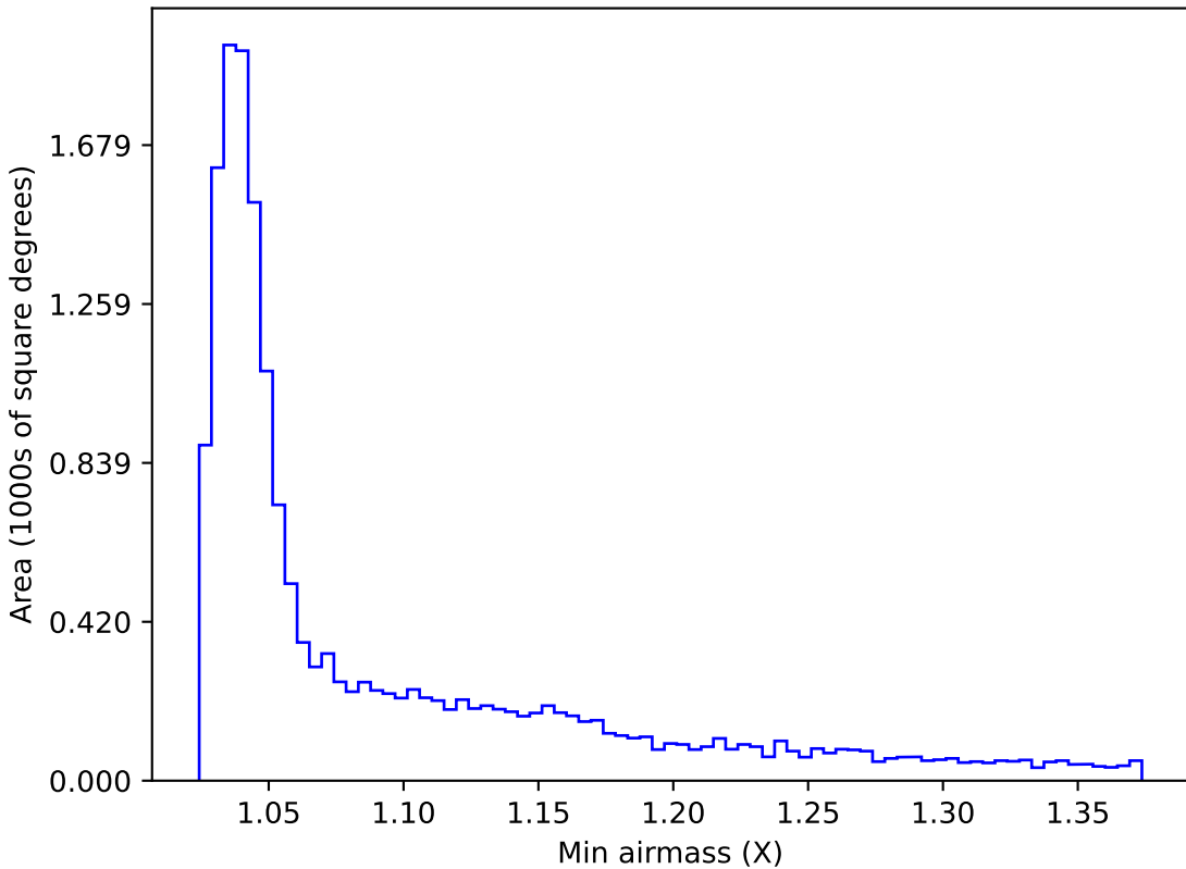
weather_cloudso31v3.4_10yrs WFD u band: Min airmass
