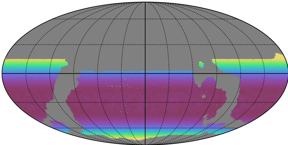
weather_cloudso31v3.4_10yrs WFD r band: Min airmass
