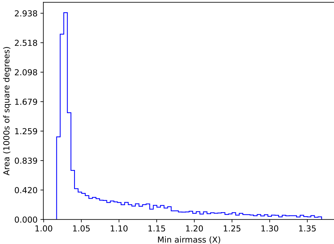
weather_cloudso31v3.4_10yrs WFD r band: Min airmass
