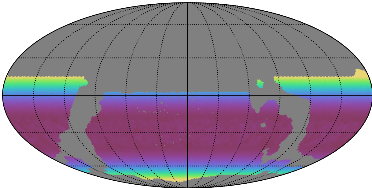
weather_cloudso31v3.4_10yrs WFD i band: Min airmass
