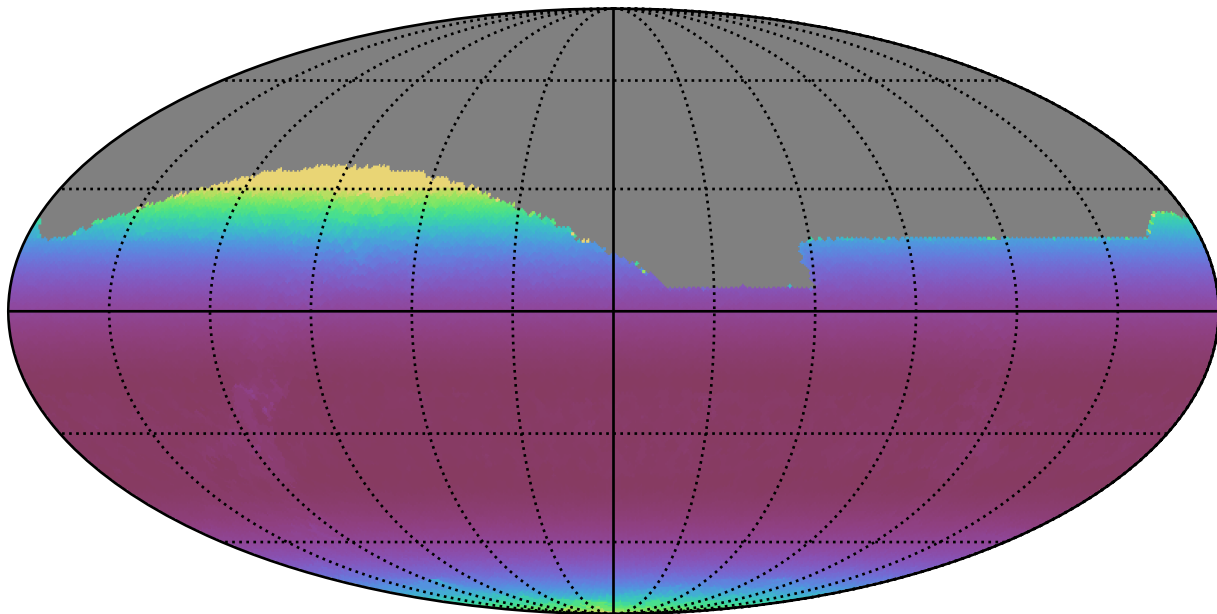
weather_cloudso31v3.4_10yrs All sky z band: Min airmass
