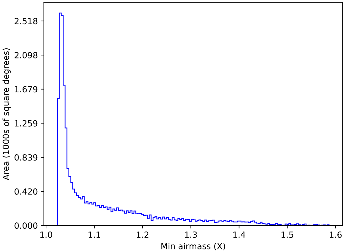
weather_cloudso31v3.4_10yrs All sky y band: Min airmass
