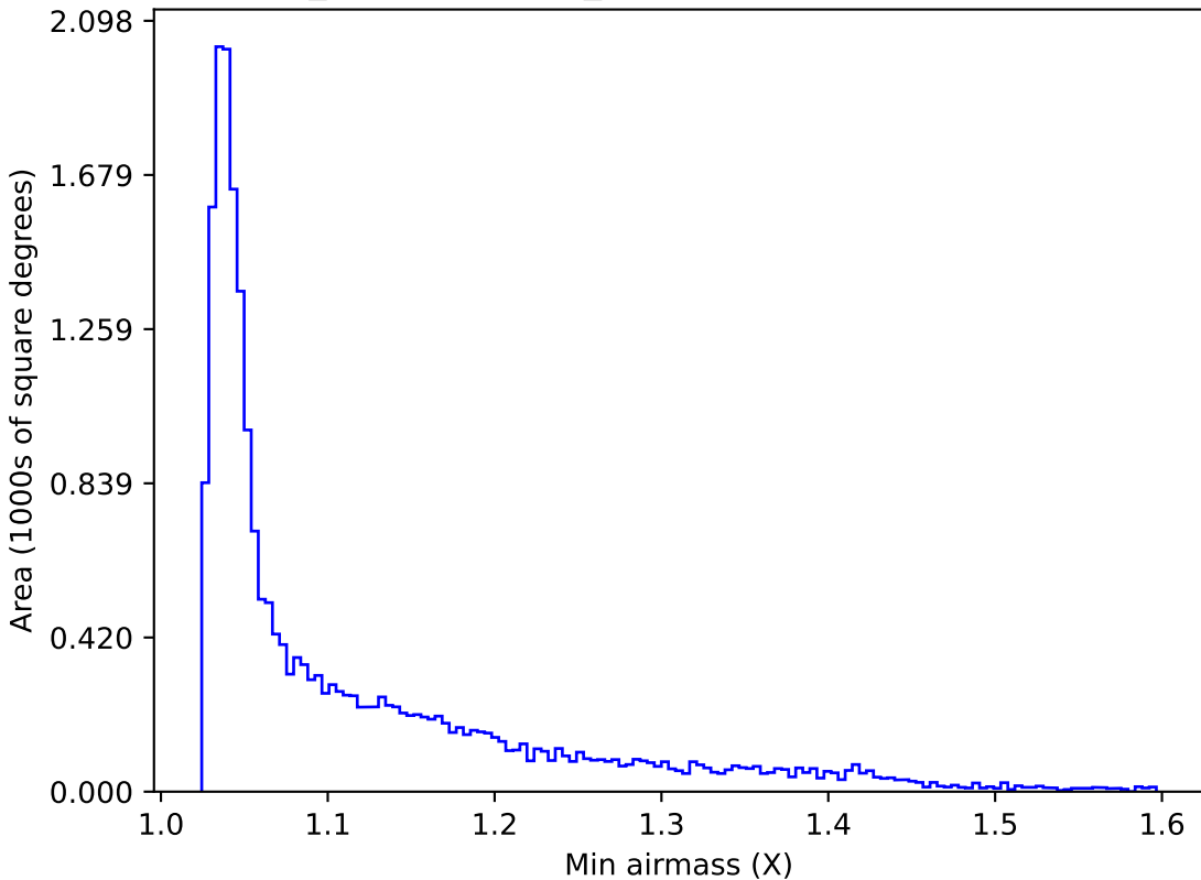
weather_cloudso31v3.4_10yrs All sky u band: Min airmass
