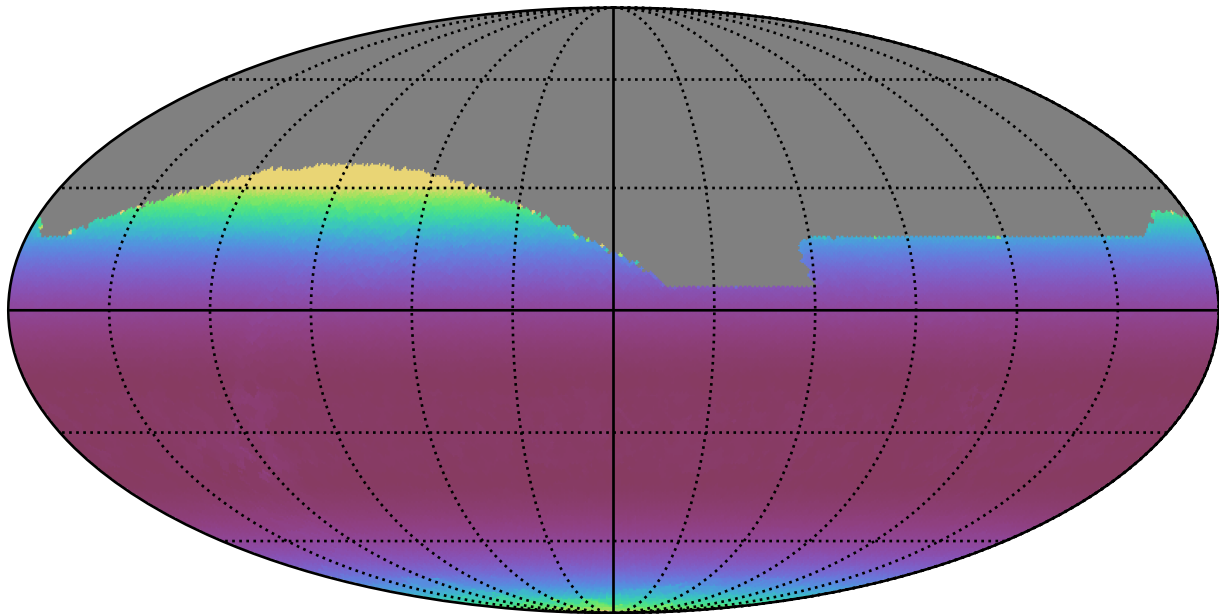
weather_cloudso31v3.4_10yrs All sky i band: Min airmass
