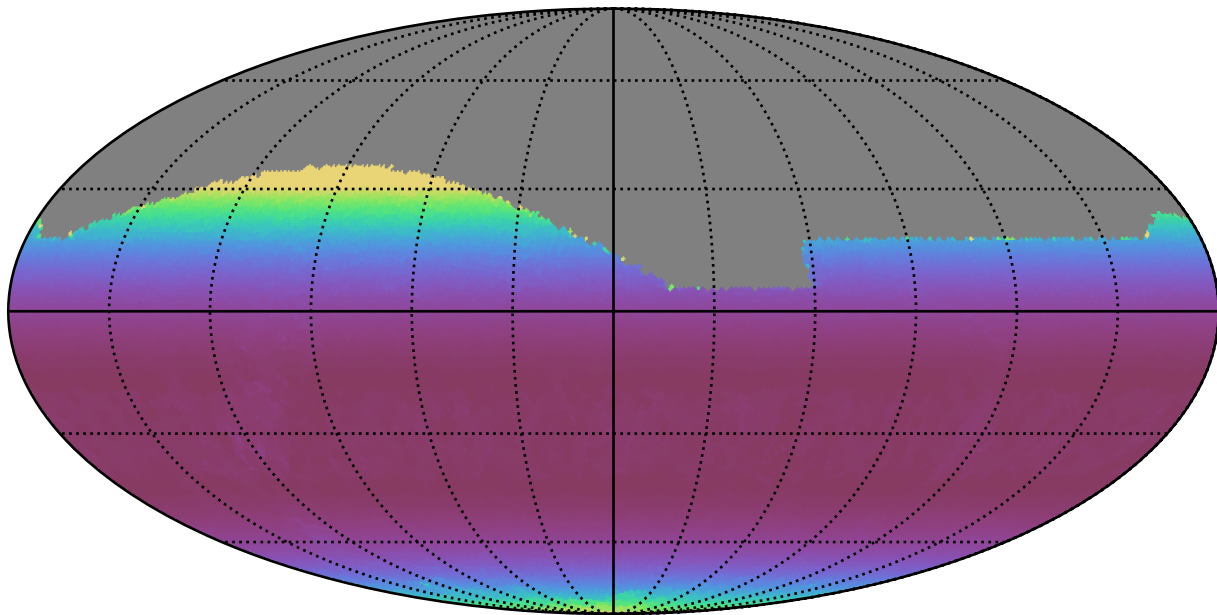
weather_cloudso31v3.4_10yrs All sky g band: Min airmass
