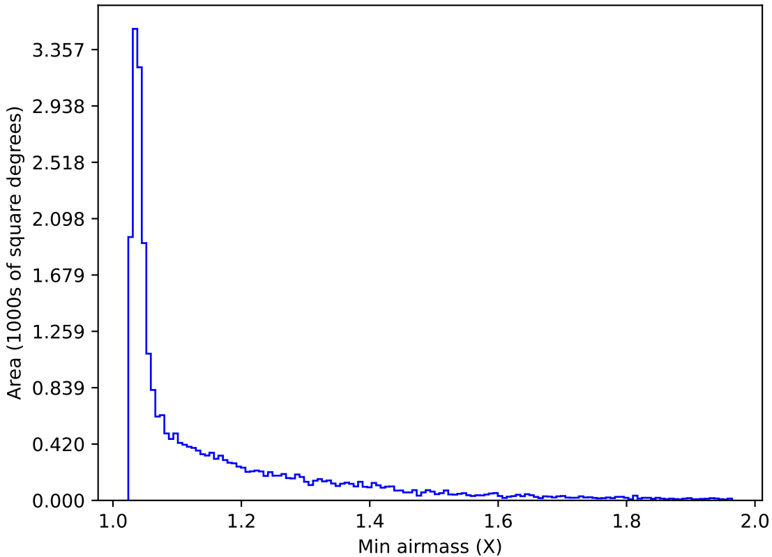
weather_cloudso31v3.4_10yrs All sky g band: Min airmass
