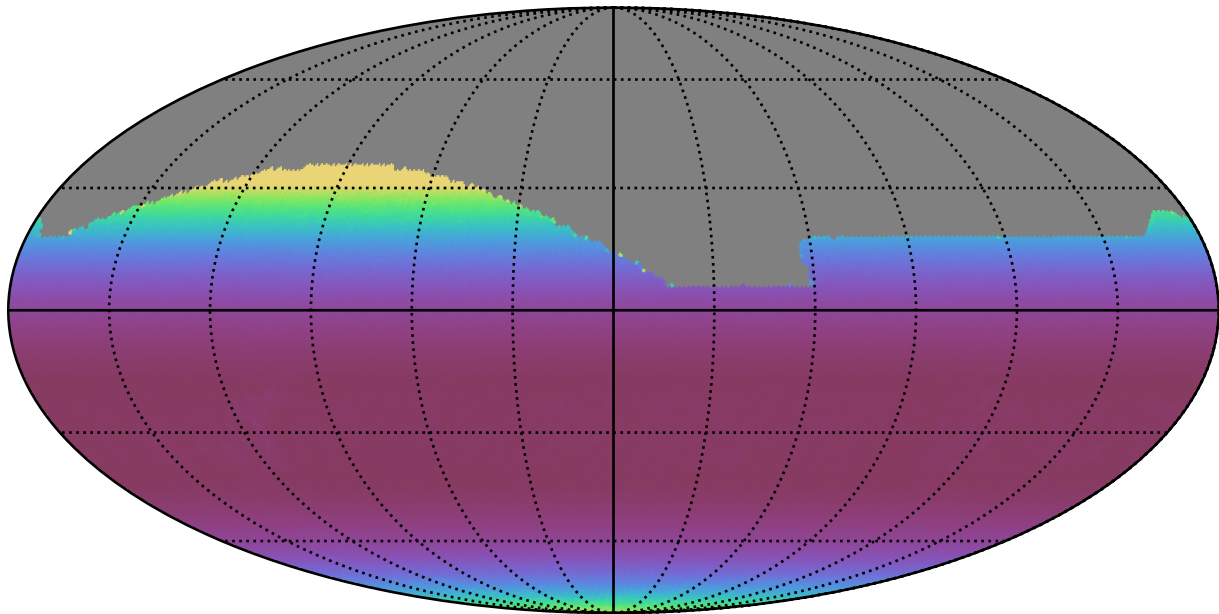
weather_cloudso31v3.4_10yrs All sky all bands: Min airmass
