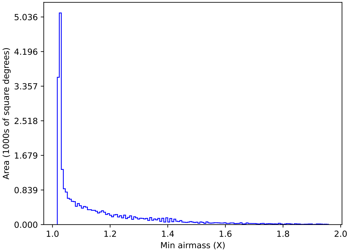
weather_cloudso31v3.4_10yrs All sky all bands: Min airmass
