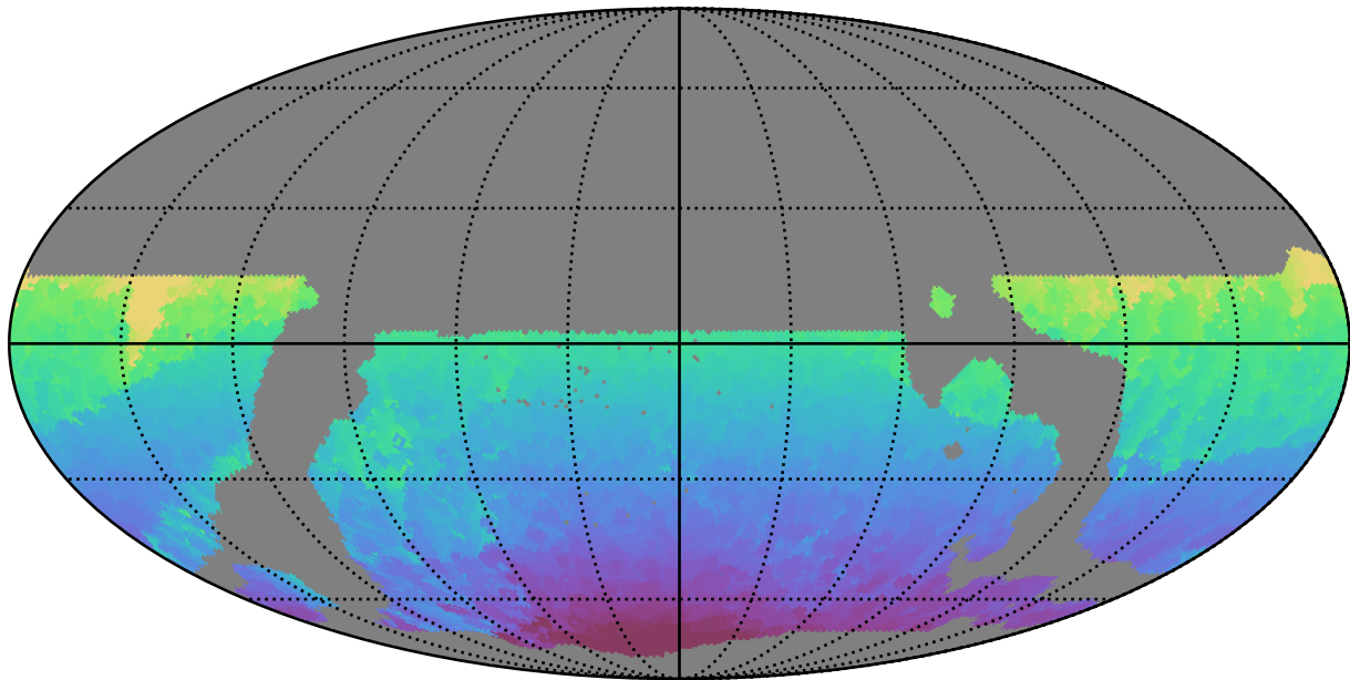
weather_cloudso31v3.4_10yrs WFD all bands: Min HA
