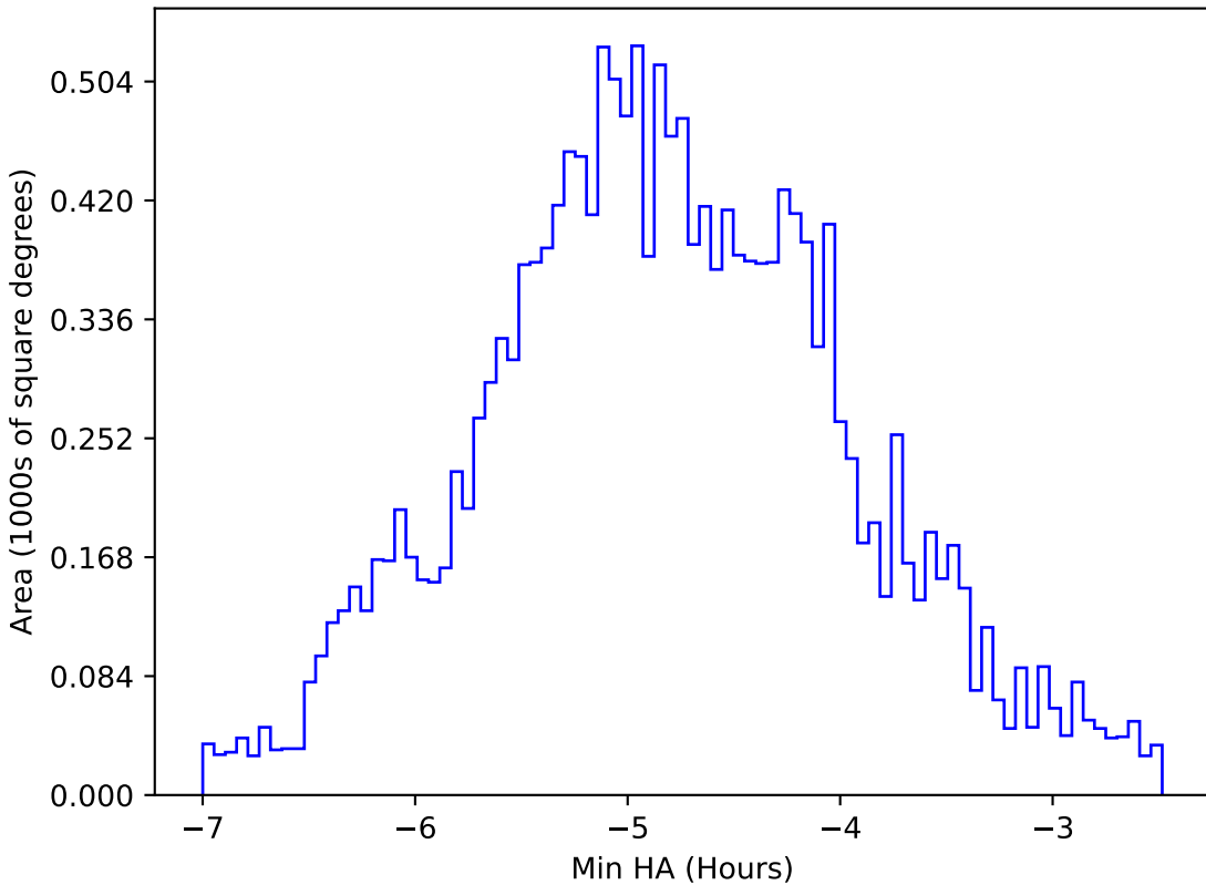
weather_cloudso31v3.4_10yrs WFD all bands: Min HA
