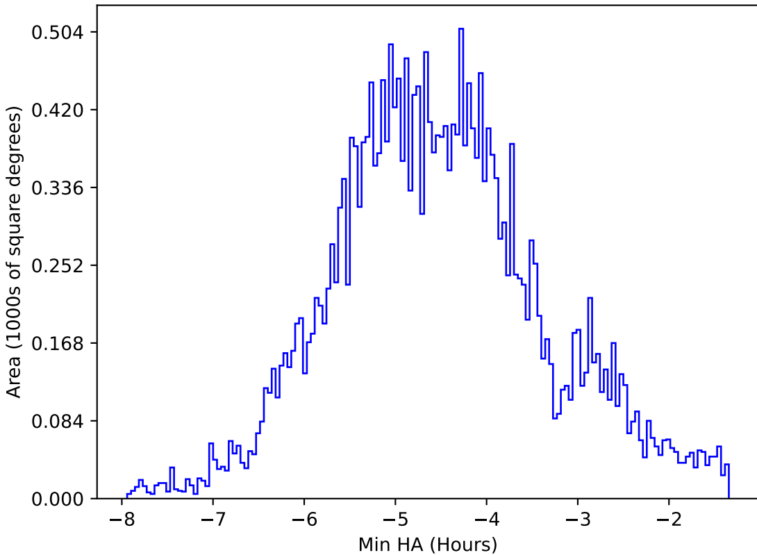
weather_cloudso31v3.4_10yrs All sky all bands: Min HA
