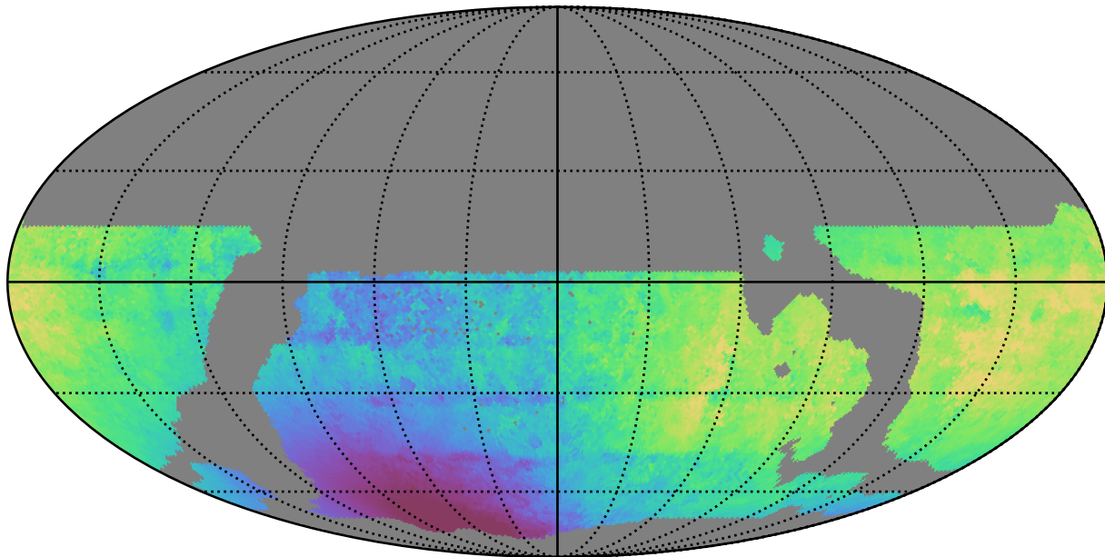
weather_cloudso31v3.4_10yrs WFD z band: Median solarElong
