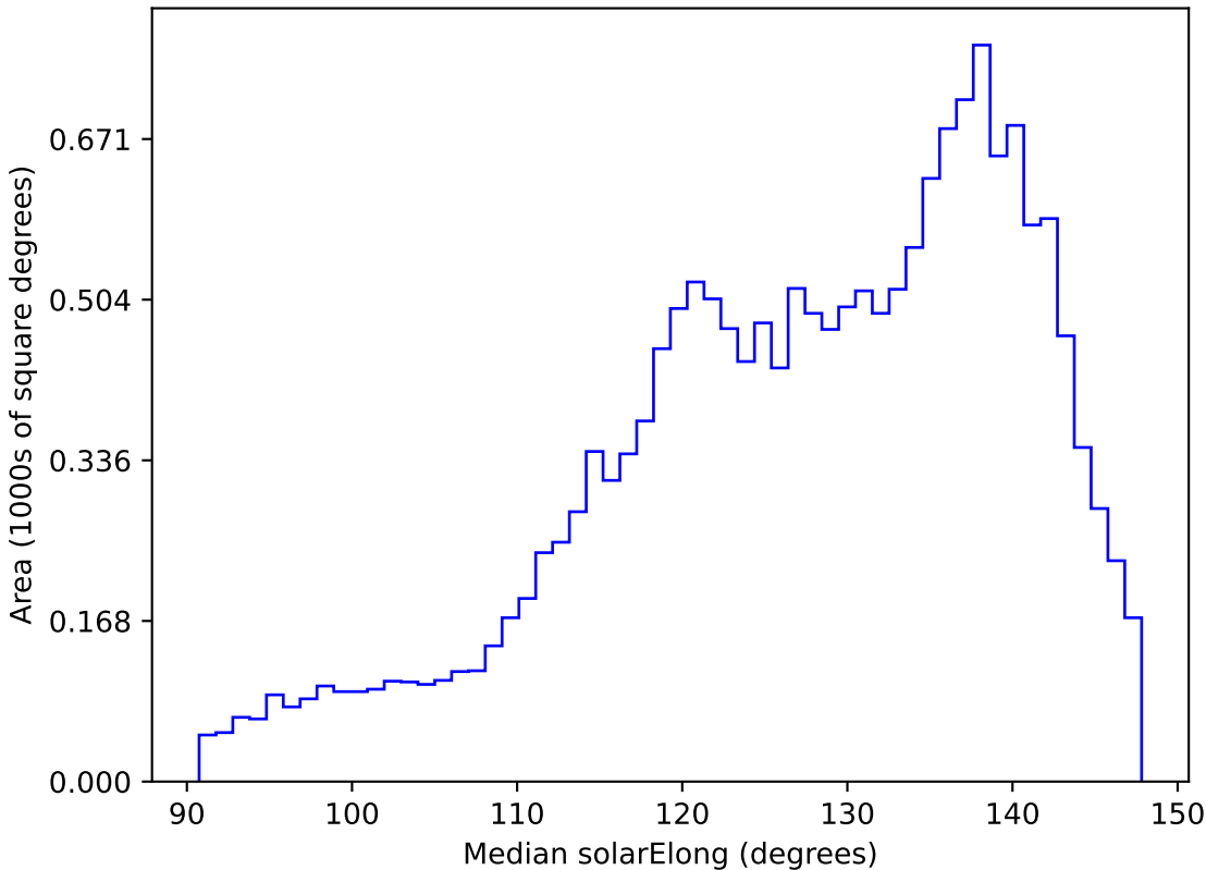
weather_cloudso31v3.4_10yrs WFD z band: Median solarElong
