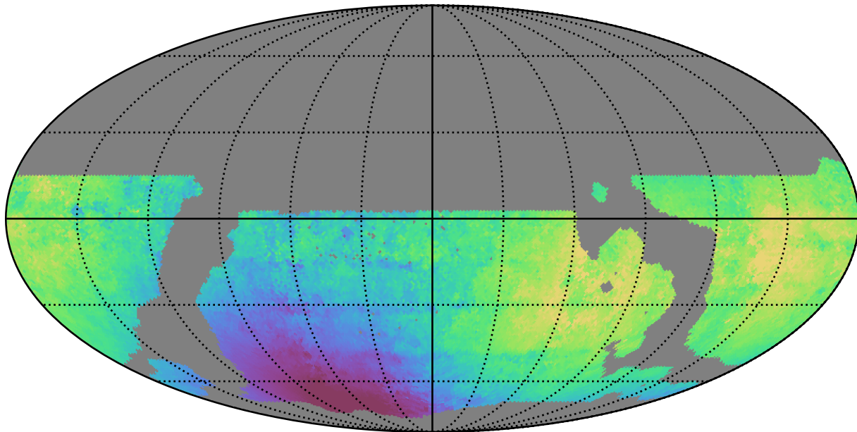
weather_cloudso31v3.4_10yrs WFD y band: Median solarElong
