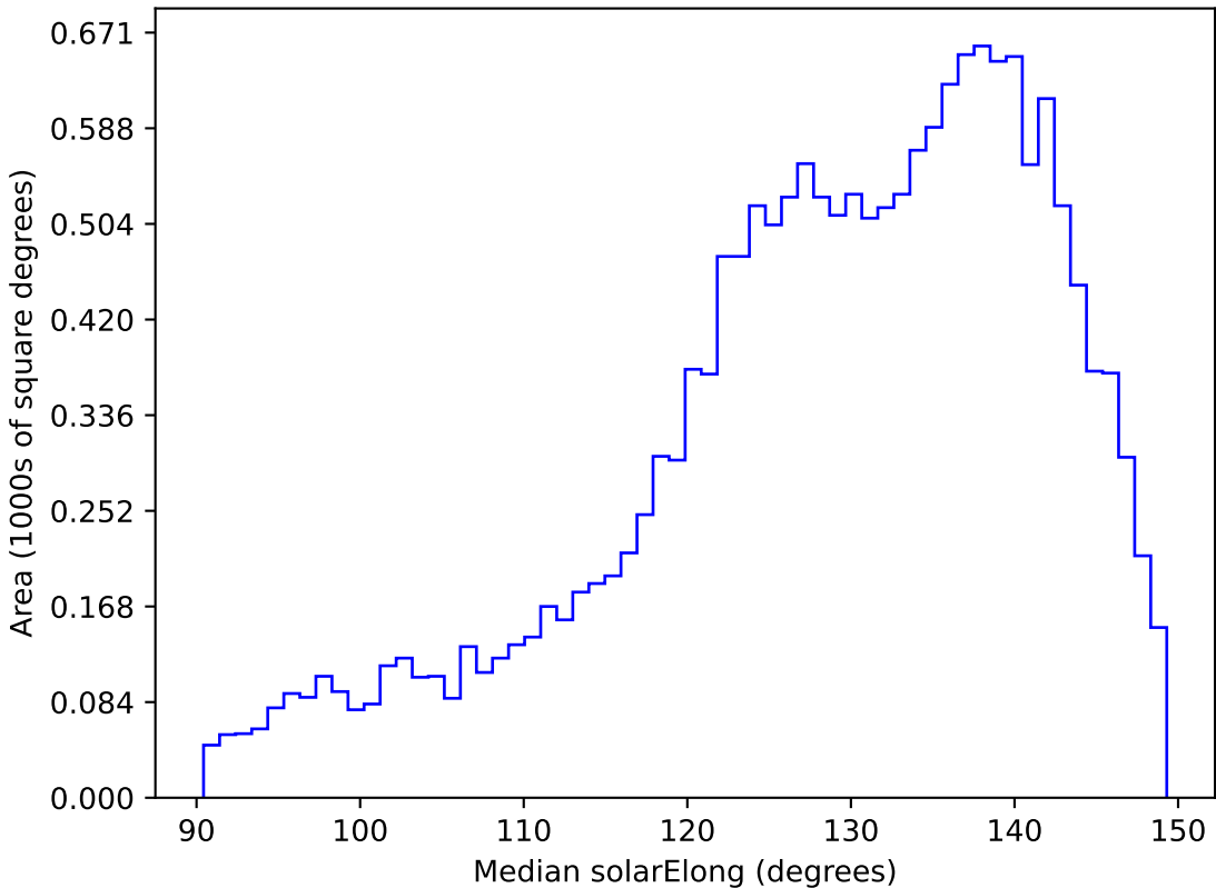
weather_cloudso31v3.4_10yrs WFD y band: Median solarElong
