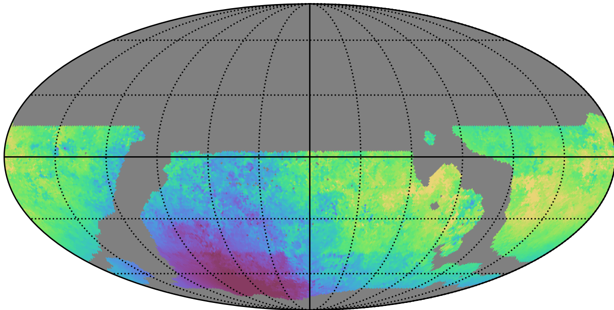
weather_cloudso31v3.4_10yrs WFD u band: Median solarElong
