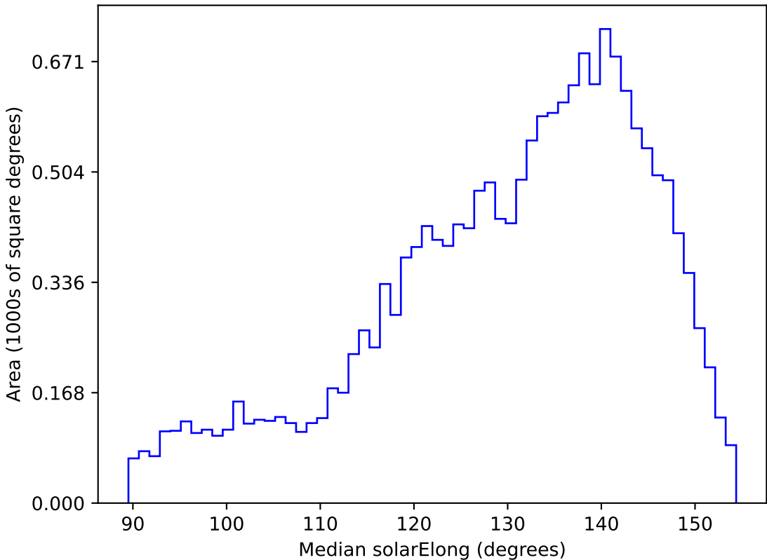
weather_cloudso31v3.4_10yrs WFD u band: Median solarElong
