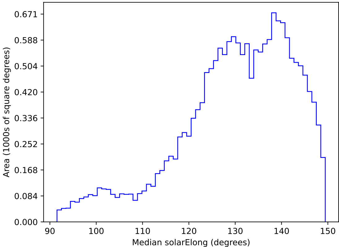
weather_cloudso31v3.4_10yrs WFD r band: Median solarElong
