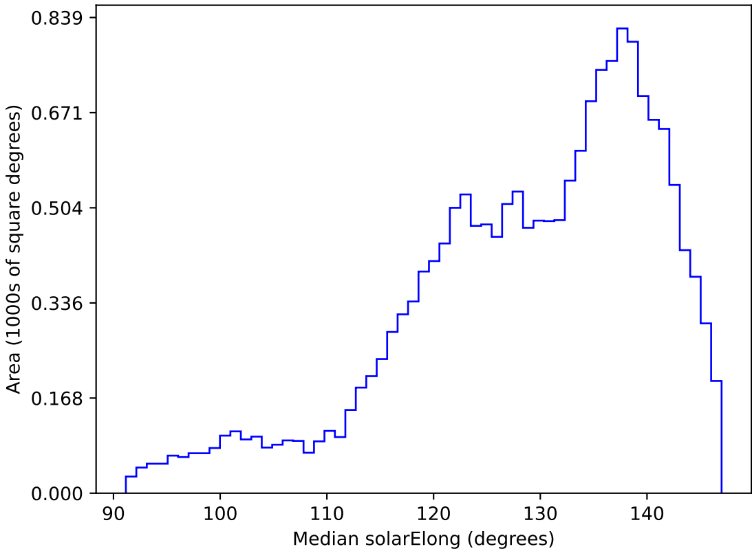
weather_cloudso31v3.4_10yrs WFD i band: Median solarElong
