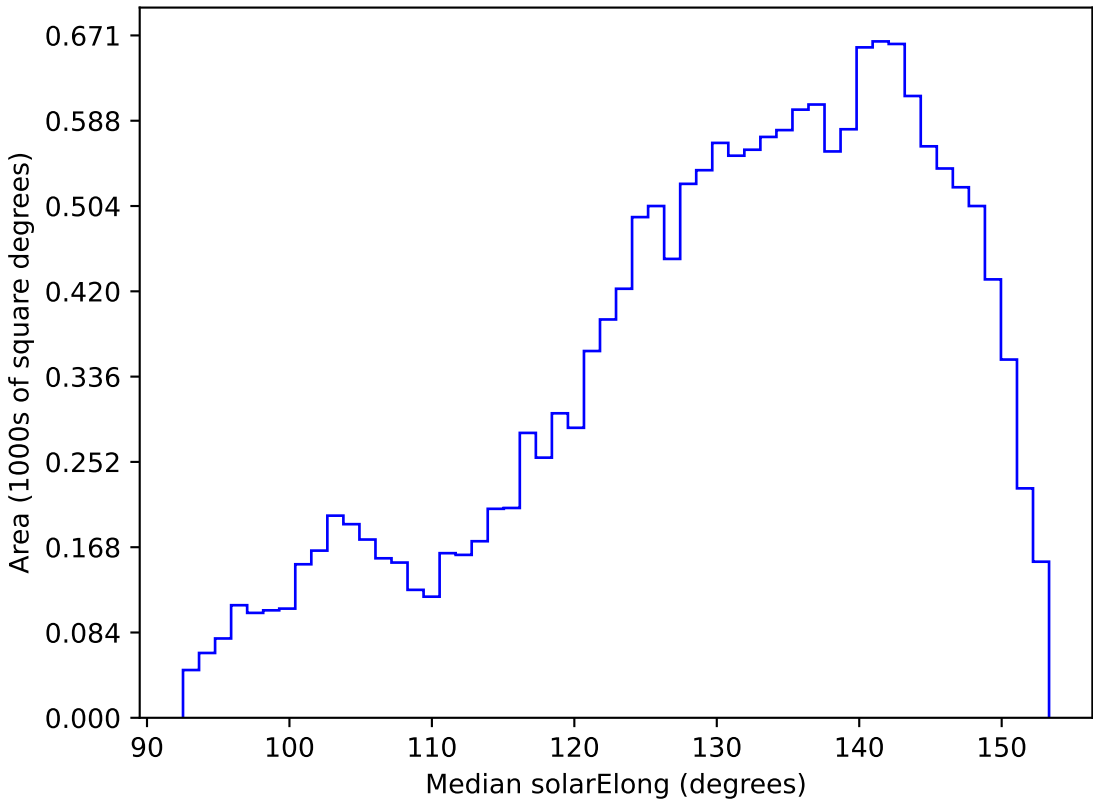
weather_cloudso31v3.4_10yrs WFD g band: Median solarElong
