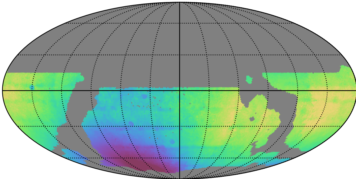
weather_cloudso31v3.4_10yrs WFD all bands: Median solarElong
