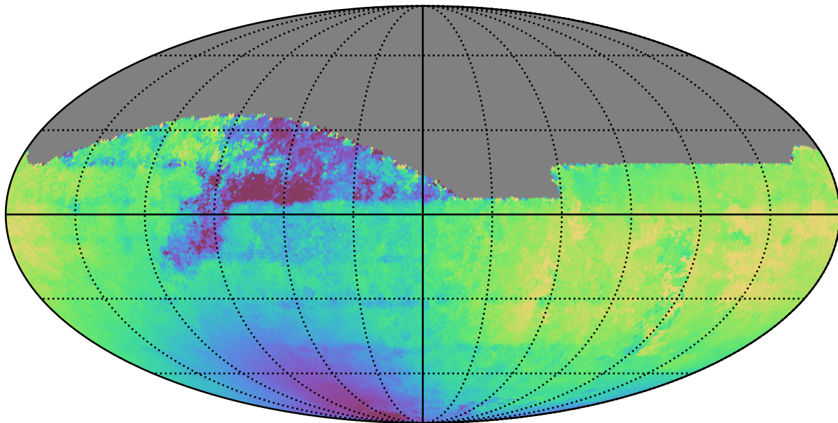
weather_cloudso31v3.4_10yrs All sky z band: Median solarElong
