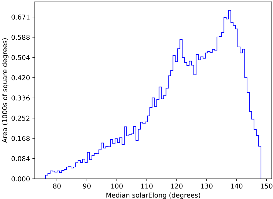
weather_cloudso31v3.4_10yrs All sky z band: Median solarElong
