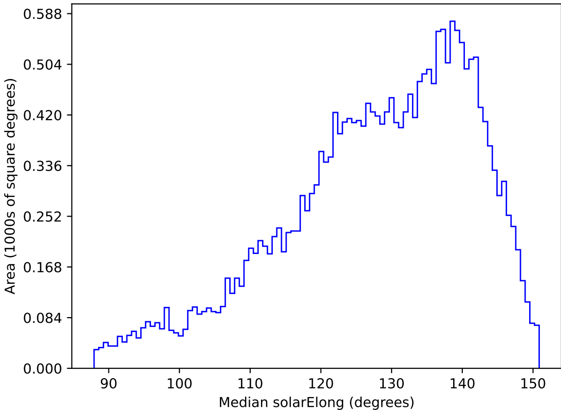
weather_cloudso31v3.4_10yrs All sky y band: Median solarElong
