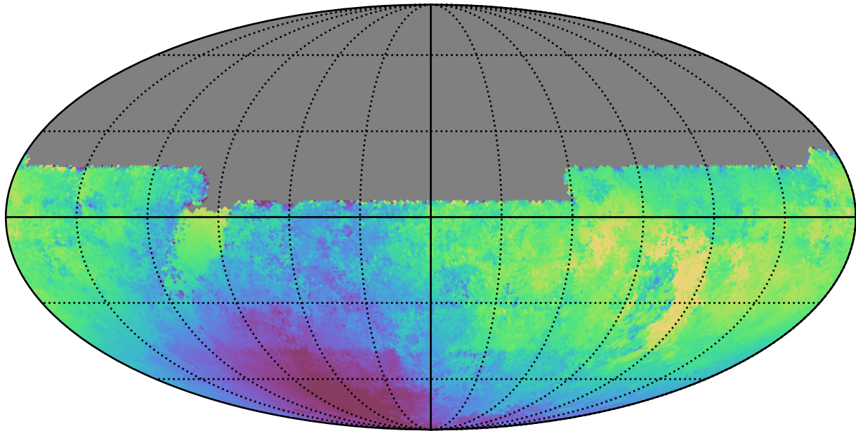
weather_cloudso31v3.4_10yrs All sky u band: Median solarElong
