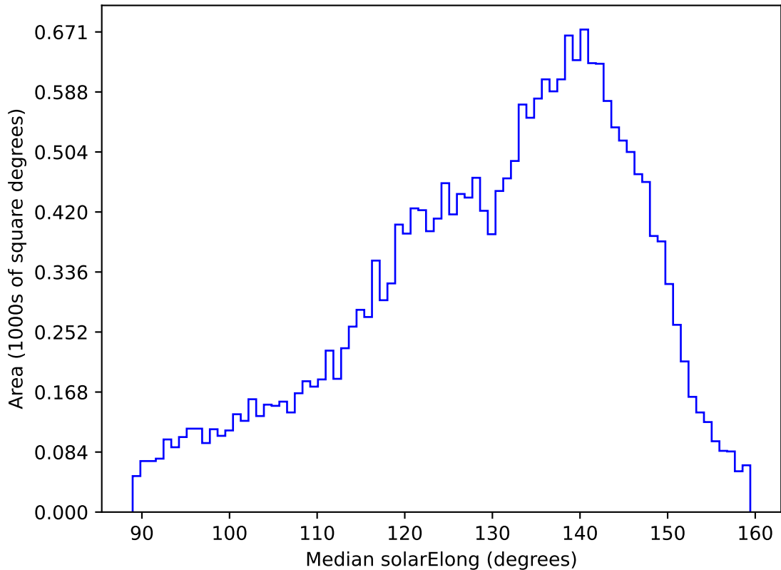
weather_cloudso31v3.4_10yrs All sky u band: Median solarElong
