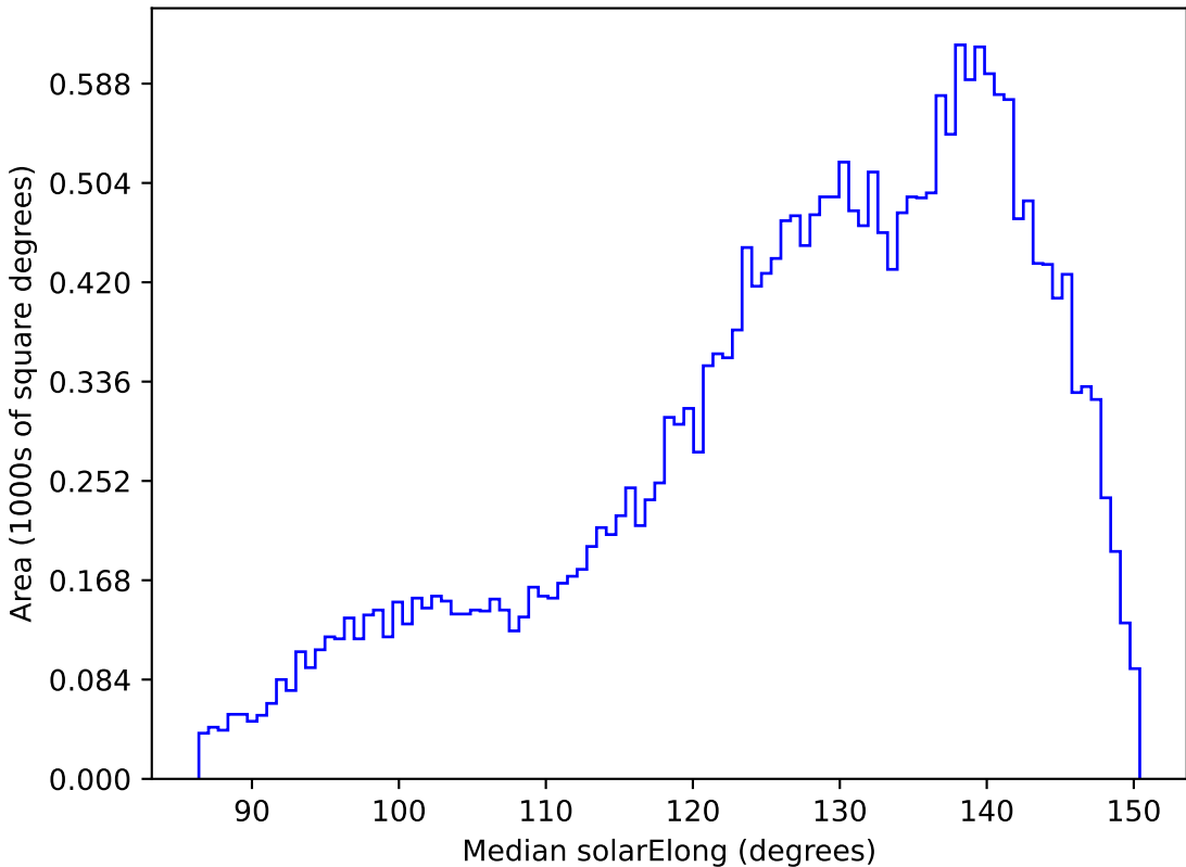
weather_cloudso31v3.4_10yrs All sky r band: Median solarElong
