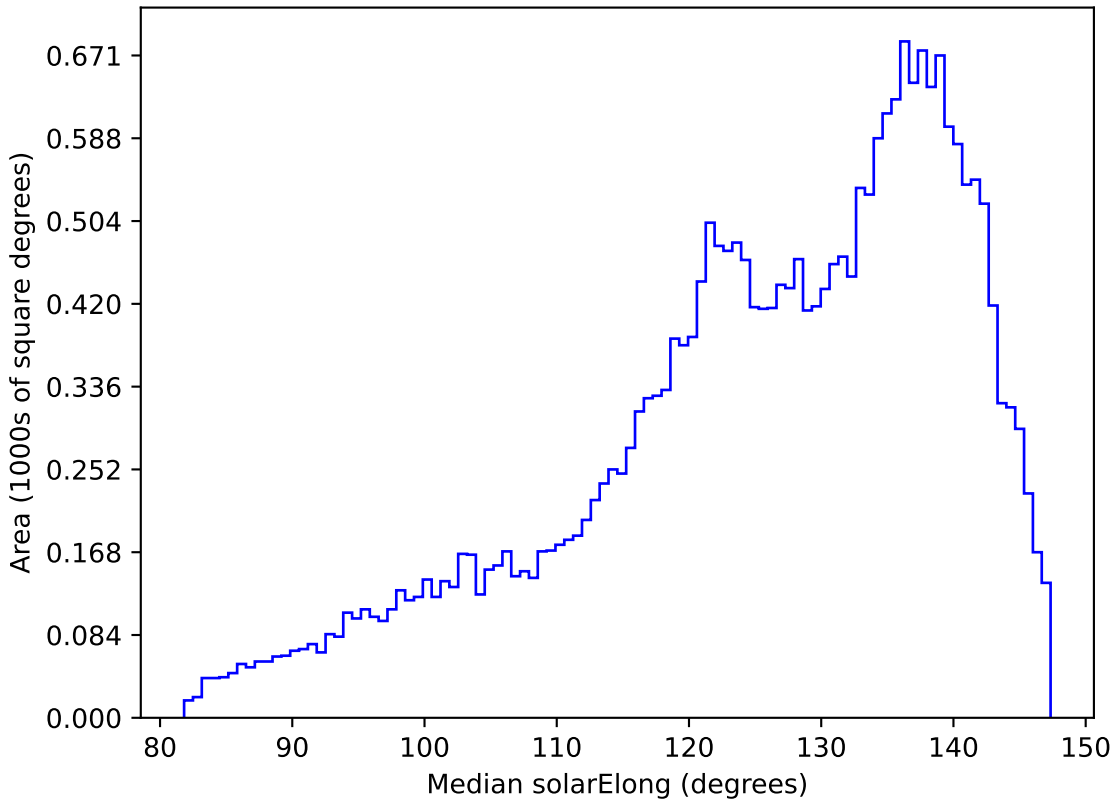
weather_cloudso31v3.4_10yrs All sky i band: Median solarElong
