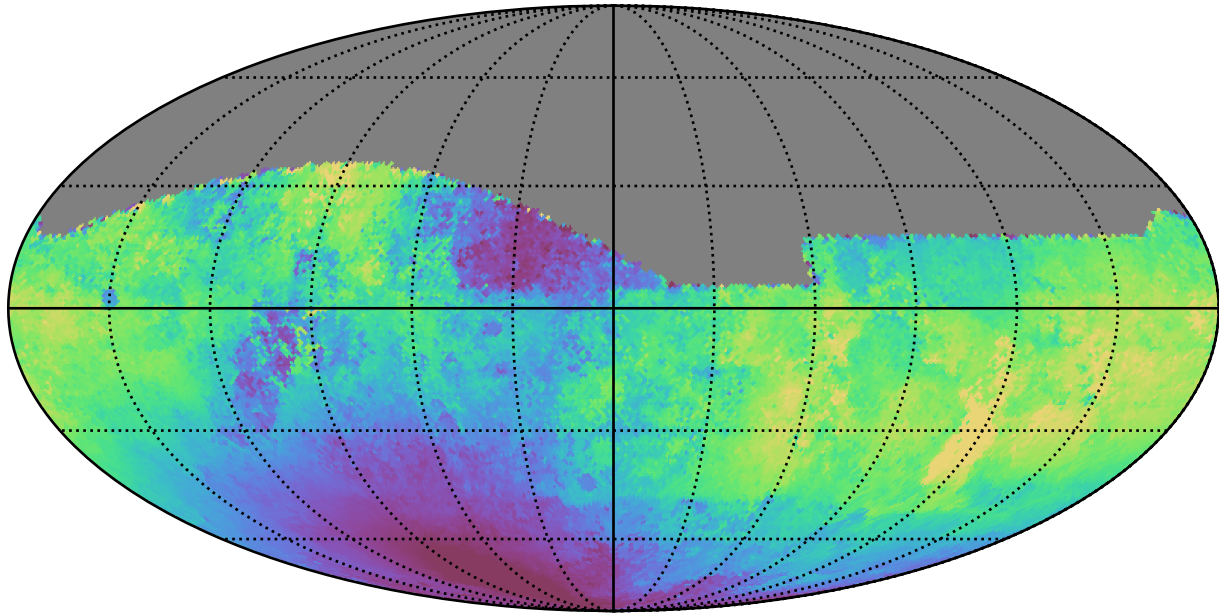
weather_cloudso31v3.4_10yrs All sky g band: Median solarElong
