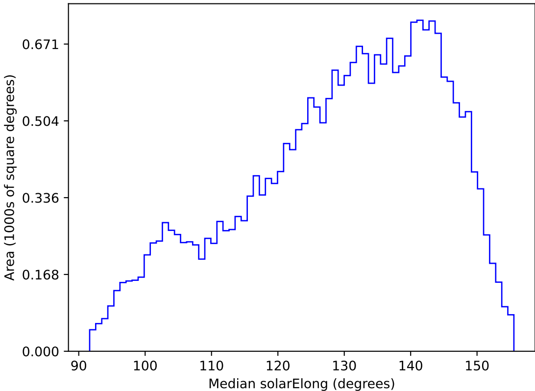
weather_cloudso31v3.4_10yrs All sky g band: Median solarElong
