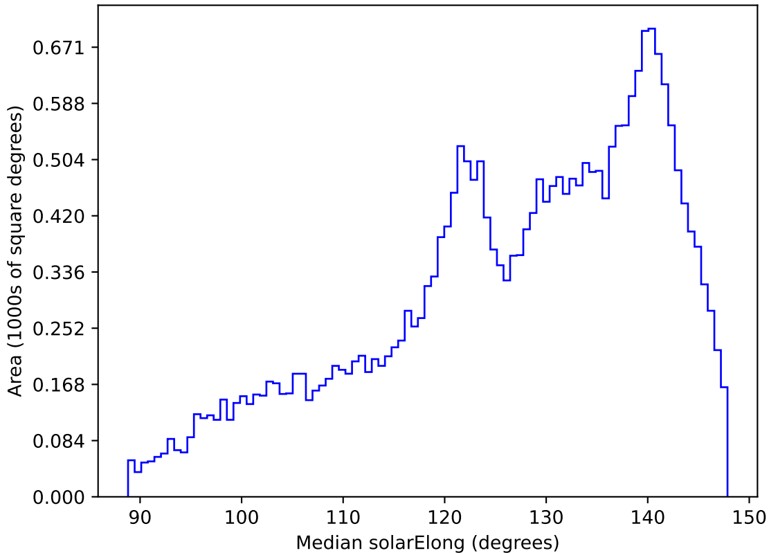
weather_cloudso31v3.4_10yrs All sky all bands: Median solarElong
