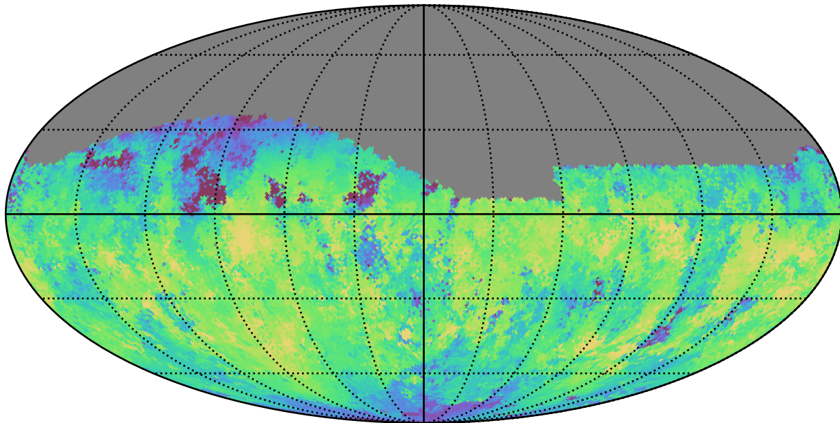
weather_cloudso31v3.4_10yrs Yr 1 z band: Median skyBrightness
