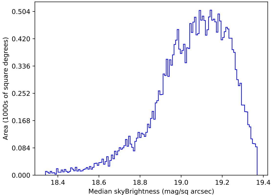
weather_cloudso31v3.4_10yrs Yr 1 z band: Median skyBrightness
