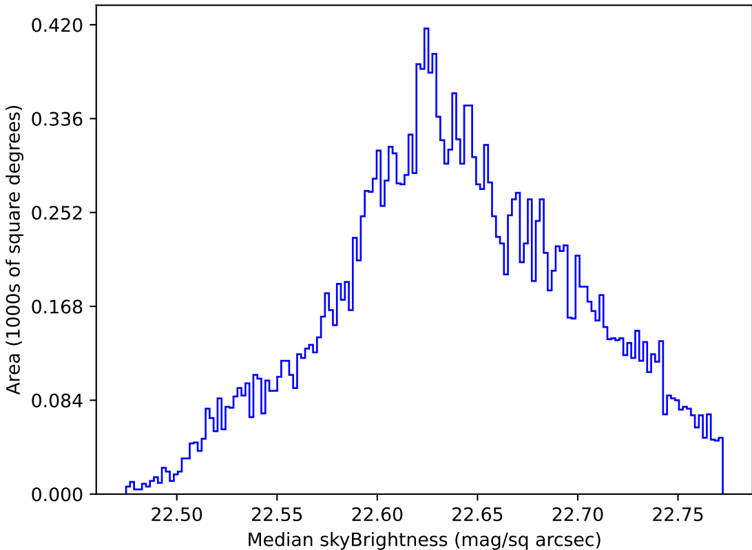
weather_cloudso31v3.4_10yrs Yr 1 u band: Median skyBrightness
