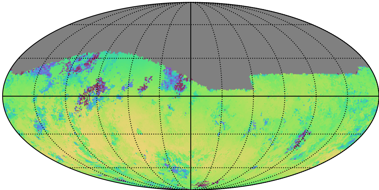
weather_cloudso31v3.4_10yrs Yr 1 r band: Median skyBrightness
