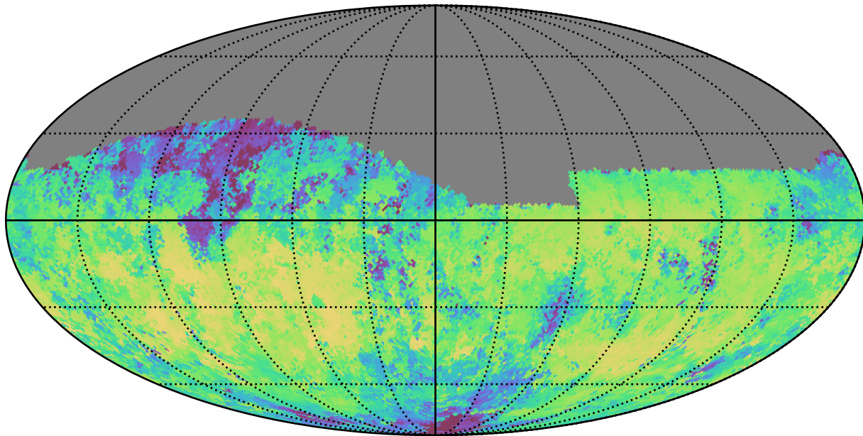
weather_cloudso31v3.4_10yrs Yr 1 i band: Median skyBrightness
