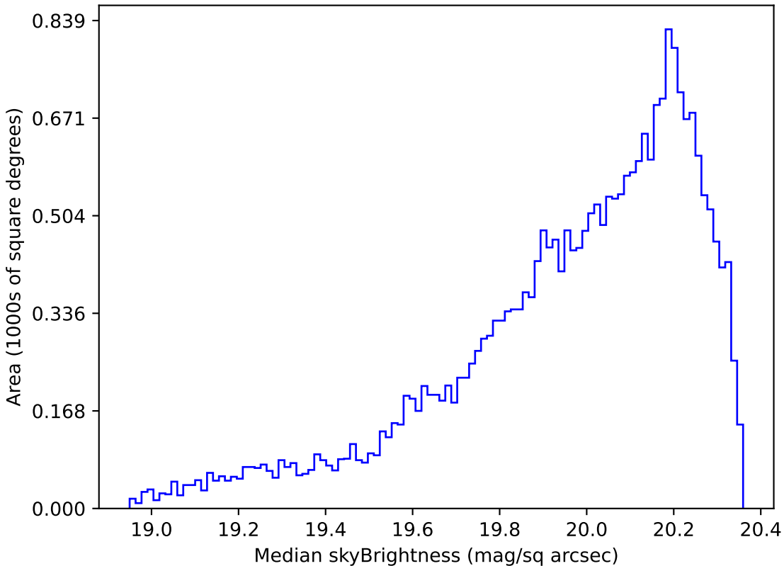
weather_cloudso31v3.4_10yrs Yr 1 i band: Median skyBrightness
