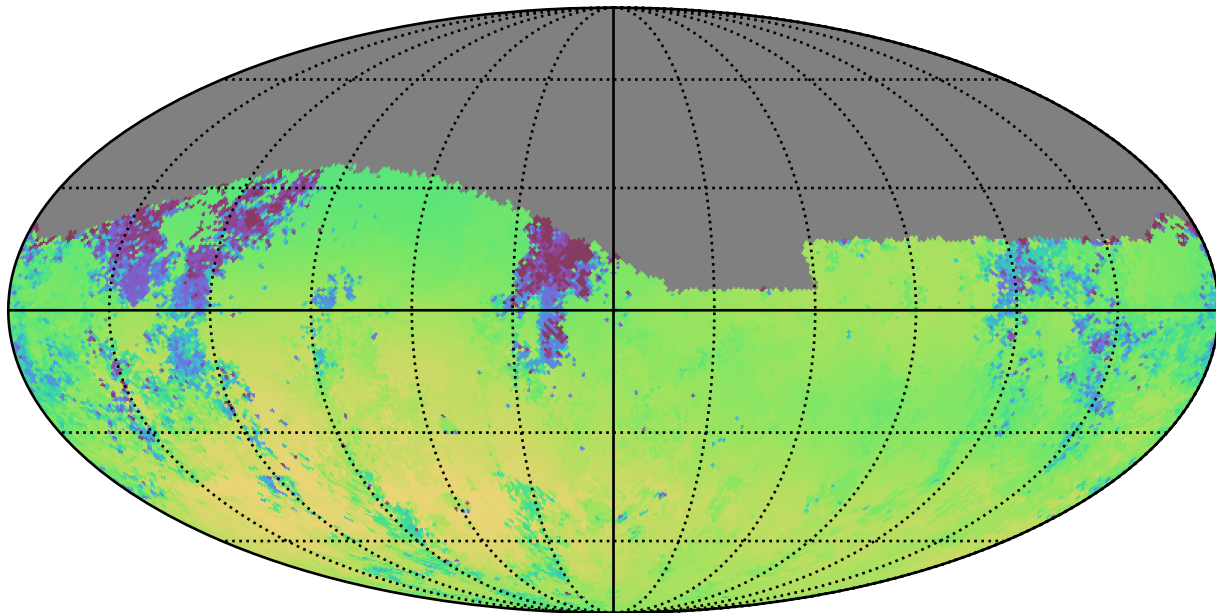
weather_cloudso31v3.4_10yrs Yr 1 g band: Median skyBrightness
