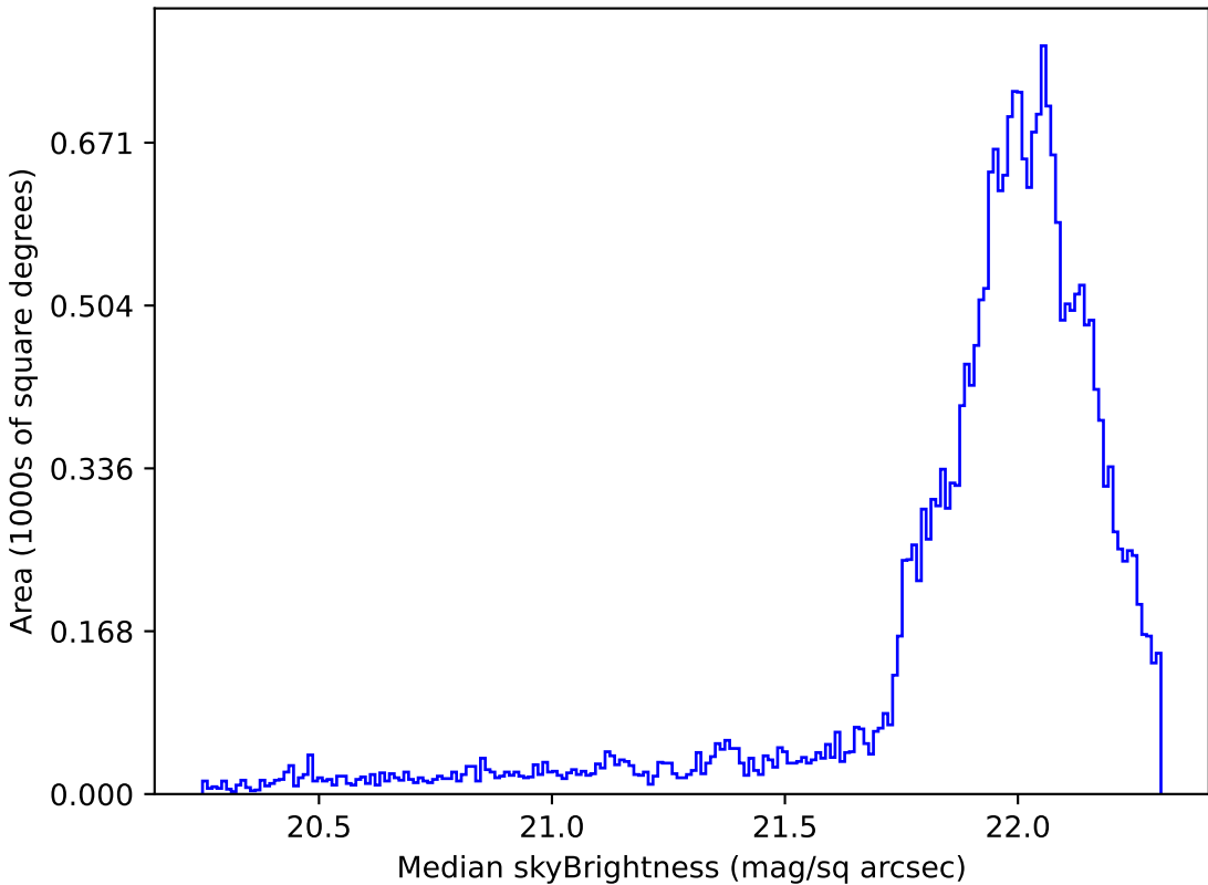
weather_cloudso31v3.4_10yrs Yr 1 g band: Median skyBrightness
