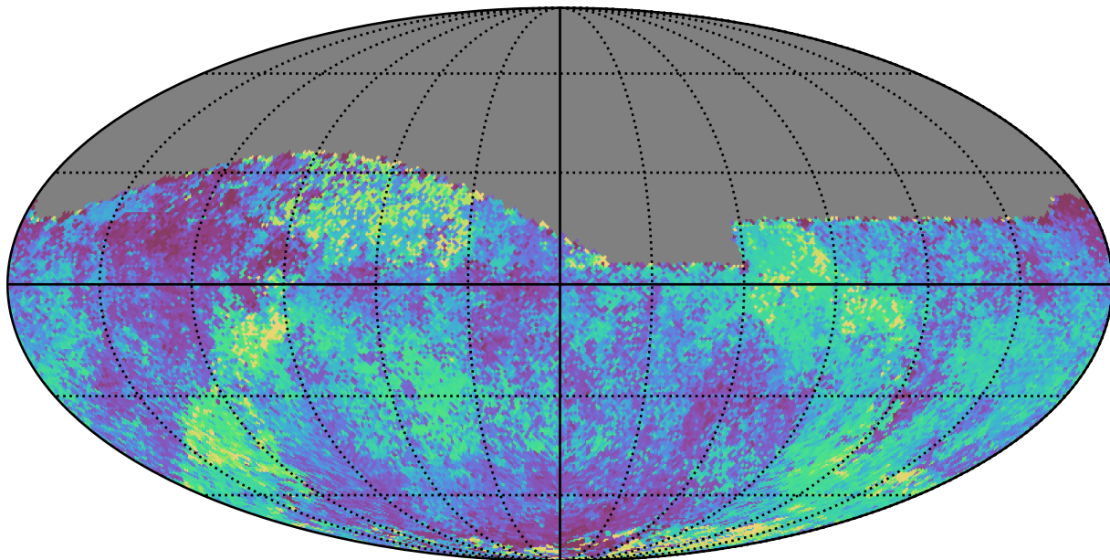
weather_cloudso31v3.4_10yrs Yr 1 all bands: Median skyBrightness
