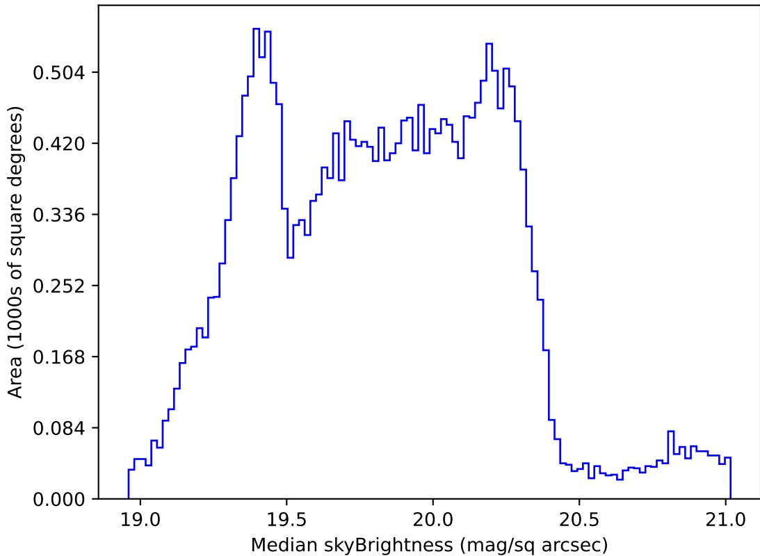
weather_cloudso31v3.4_10yrs Yr 1 all bands: Median skyBrightness
