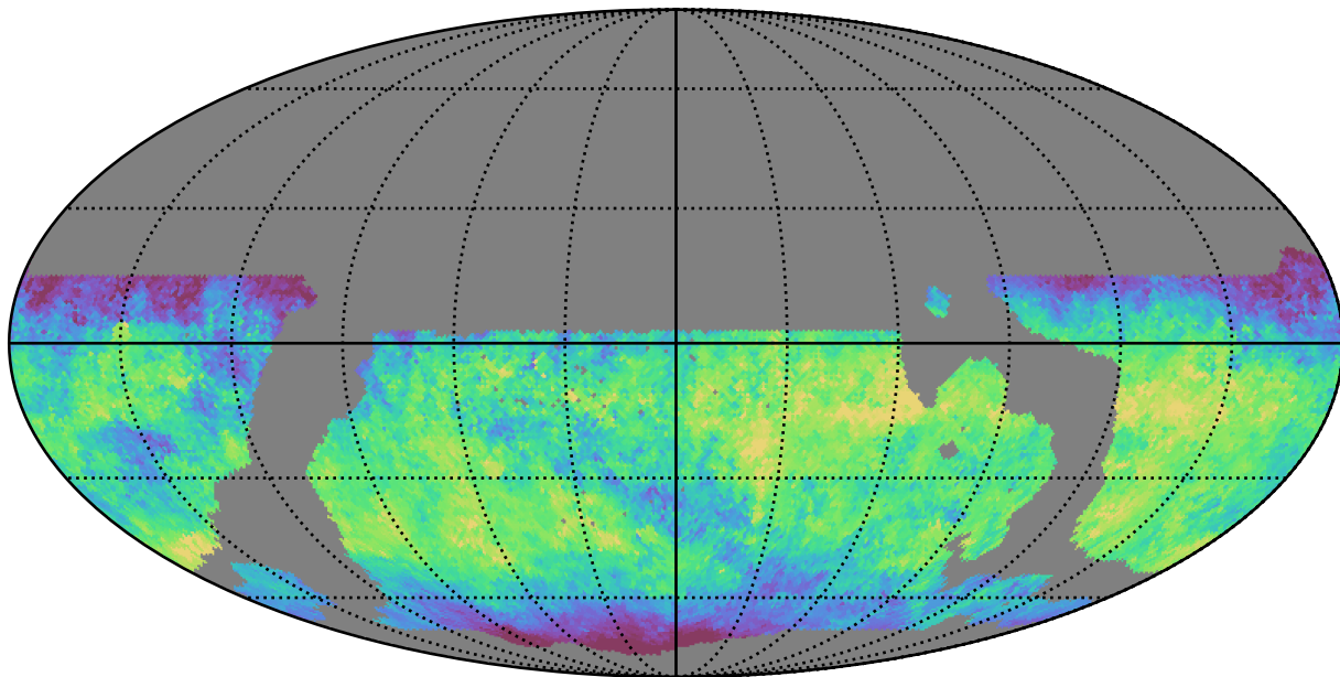
weather_cloudso31v3.4_10yrs WFD z band: Median skyBrightness
